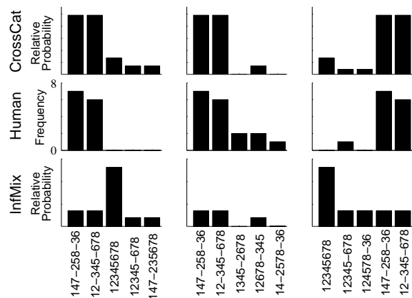
Figure 5: Results from the 3-3 condition. In each column, the results are sorted by a different standard: from left to right, the results are sorted by CrossCat predictions, human results, and the infinite mixture model's predictions. Note that the y-axis scale is the same across each row and the model solutions are plotted according to their relative probability, while the human data are plotted by frequency. On the x-axis is the partition of the objects, with different categories separated by dashes. For example, in the case at the far left, stimuli 1, 4, and 7 were in the same category, while stimuli 2, 5, and 8 were in another.
