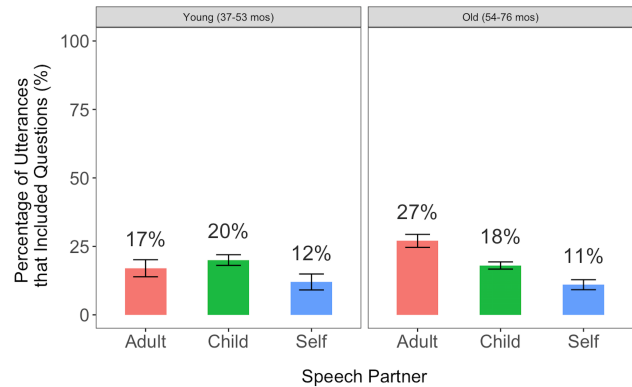
Figure 3: Proportion of utterances including questions as a function of speech partner in younger age group (left) or older age group (right). Older children asked more questions to adults than other children or themselves. Error bars denote SE .
